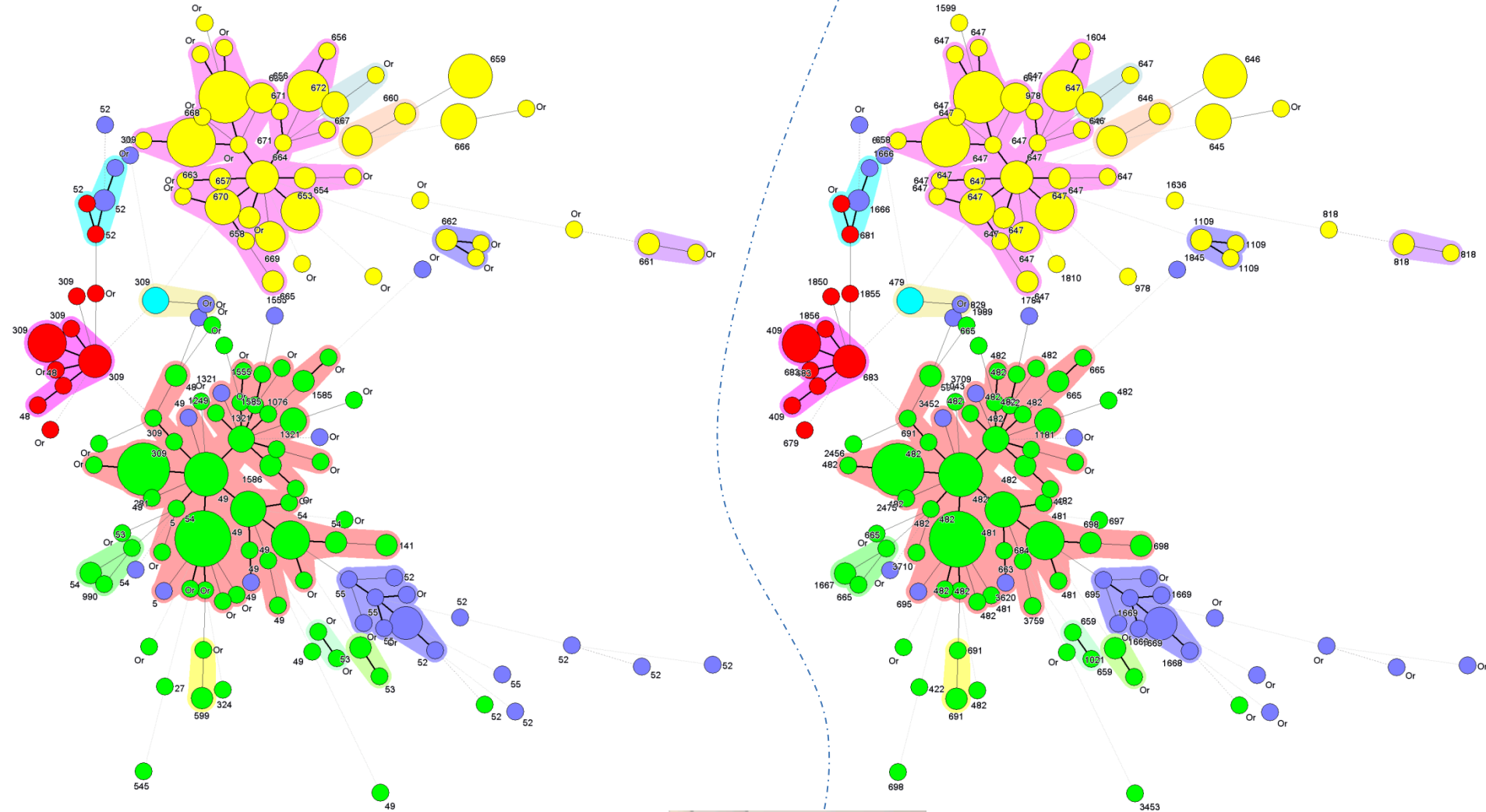
A. MST of spoligotypes in conjunction with 12-loci MIRU-VNTRs vs. sublineages. 12-MIT numbers are indicated.
